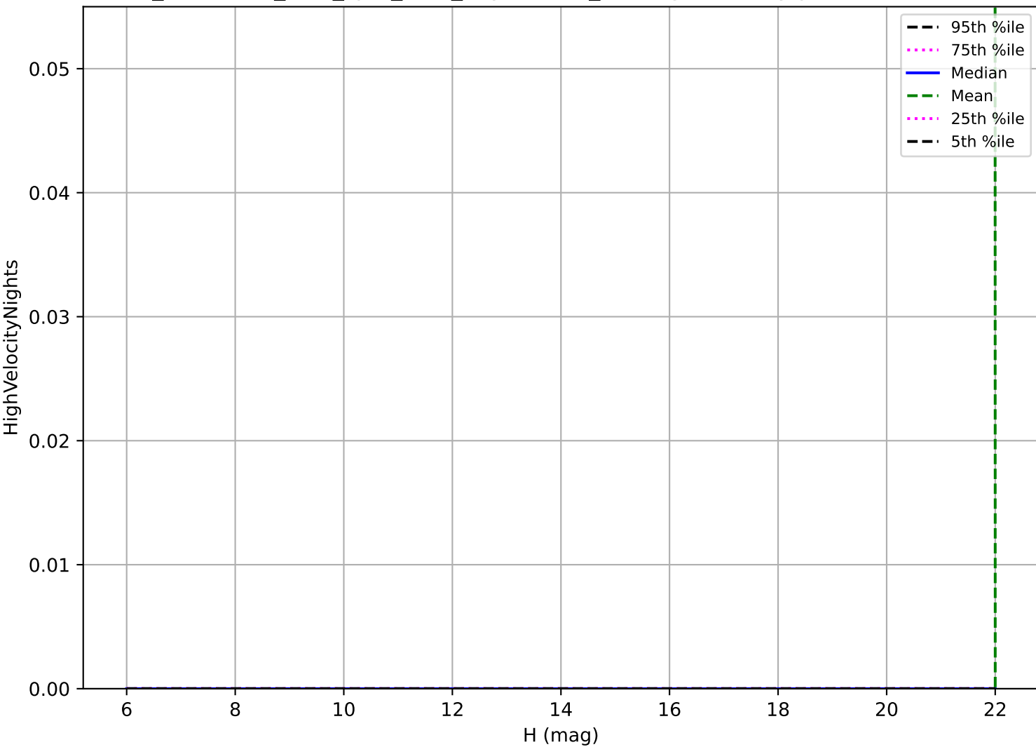
too_combined_s1.0_split_v3.4_10yrs: OCC_r20 High velocity pair detection loss
