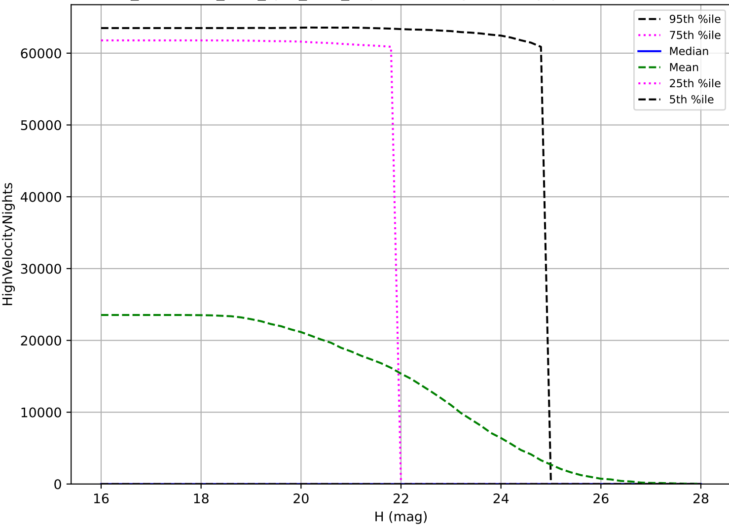
too_combined_s1.0_split_v3.4_10yrs: NEO High velocity pair detection loss
