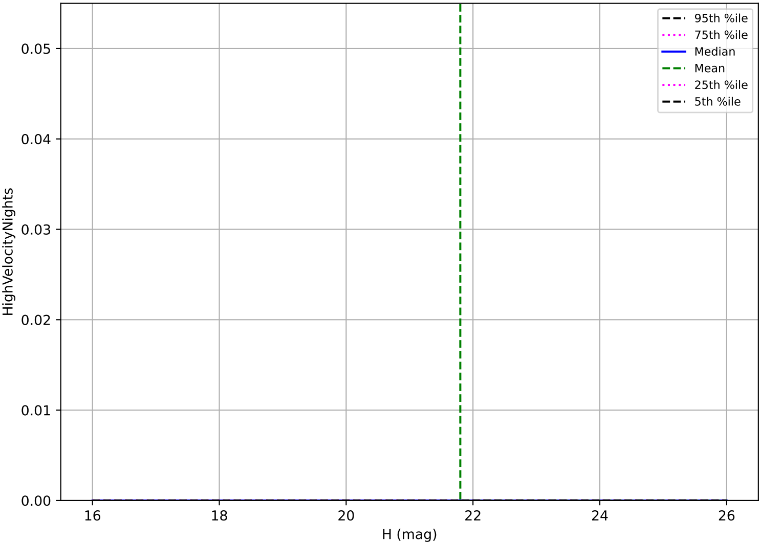
too_combined_s1.0_split_v3.4_10yrs: MBA High velocity pair detection loss
