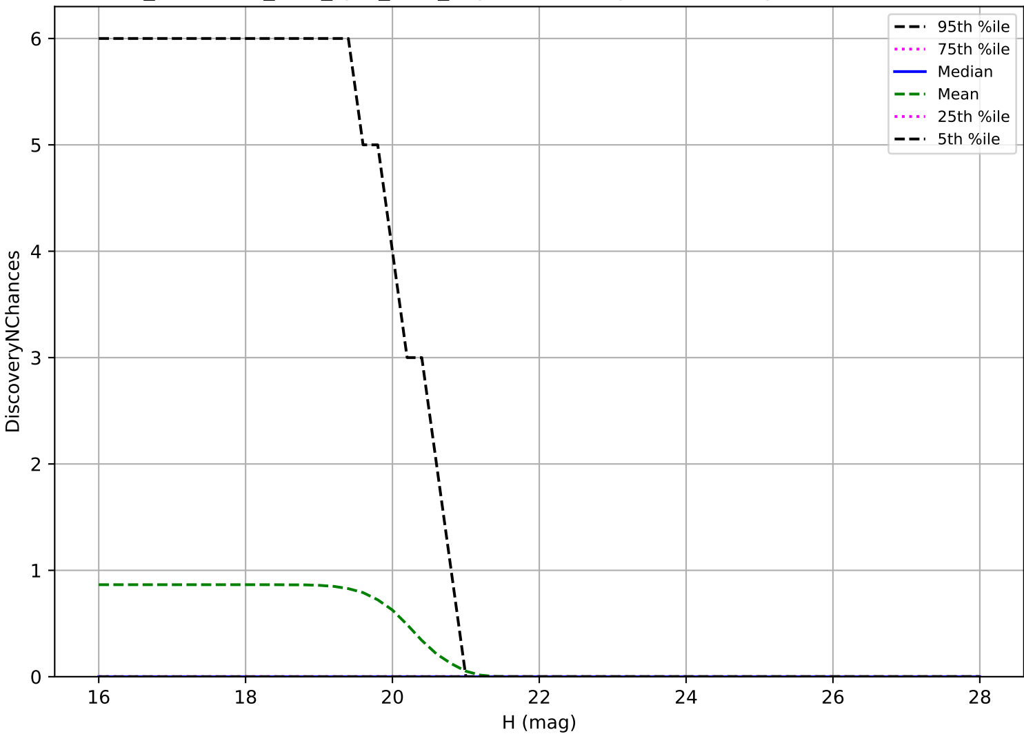
too_combined_s1.0_split_v3.4_10yrs: Vatira 3 pairs in 15 nights detection loss
