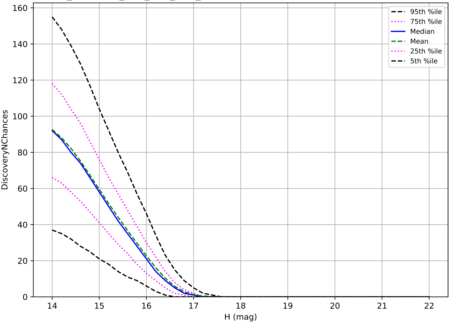
too_combined_s1.0_split_v3.4_10yrs: Trojan 3 pairs in 15 nights detection loss
