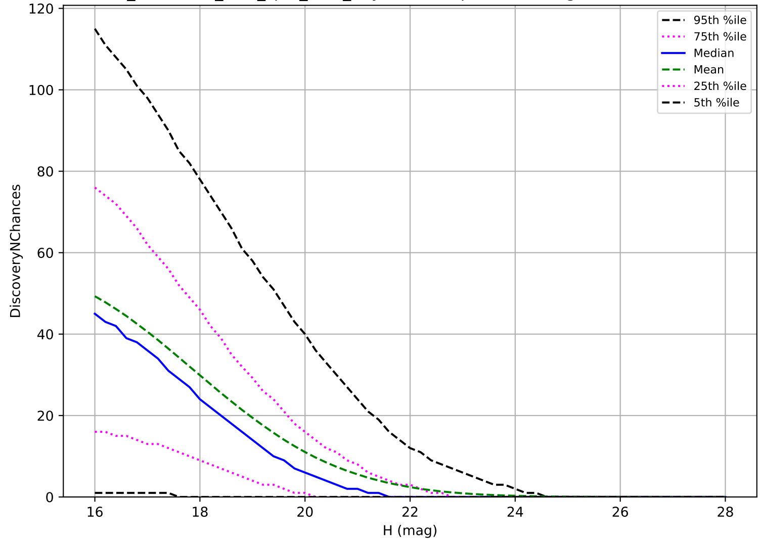
too_combined_s1.0_split_v3.4_10yrs: PHA 3 pairs in 15 nights detection loss
