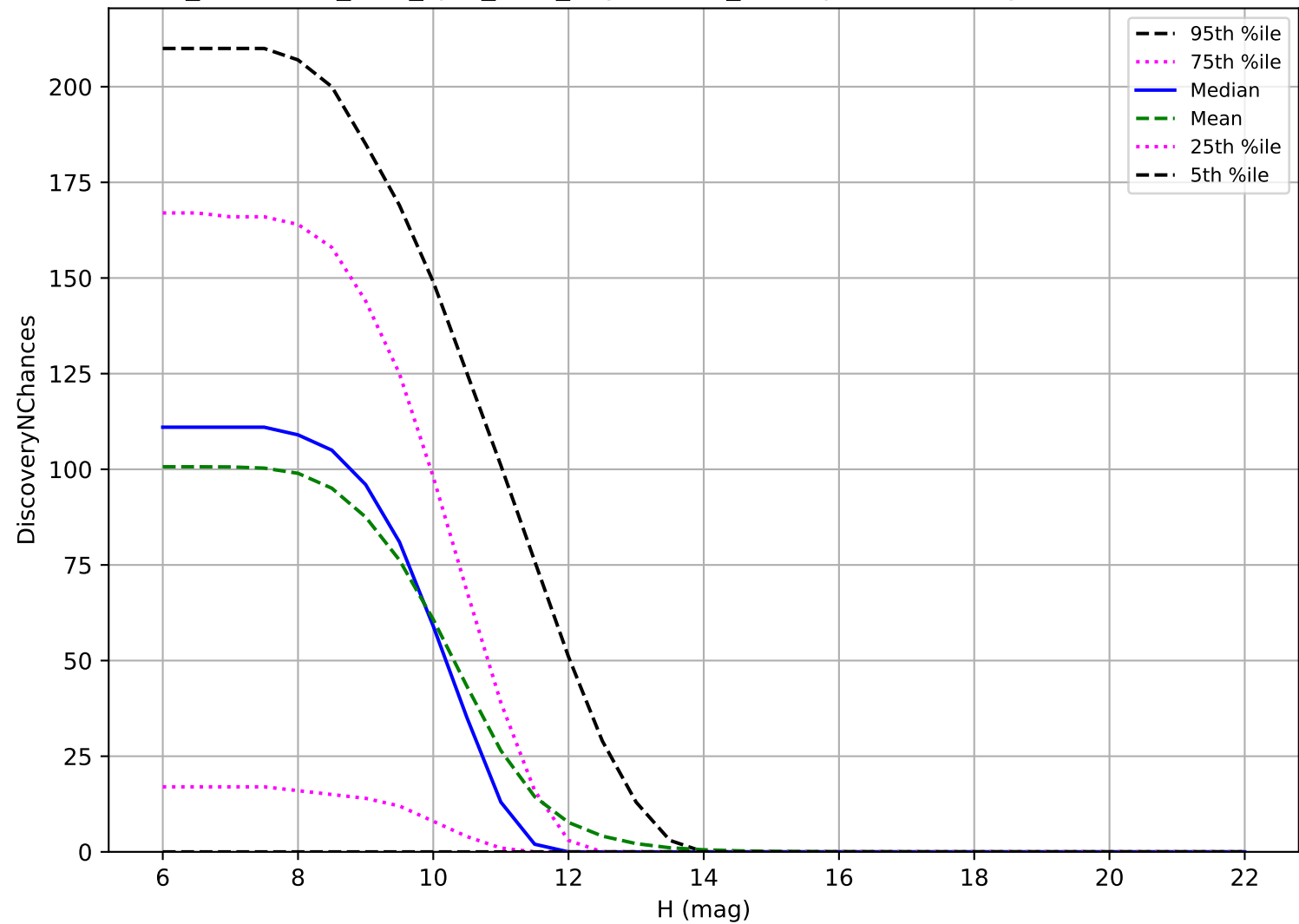
too_combined_s1.0_split_v3.4_10yrs: OCC_r20 3 pairs in 15 nights detection loss
