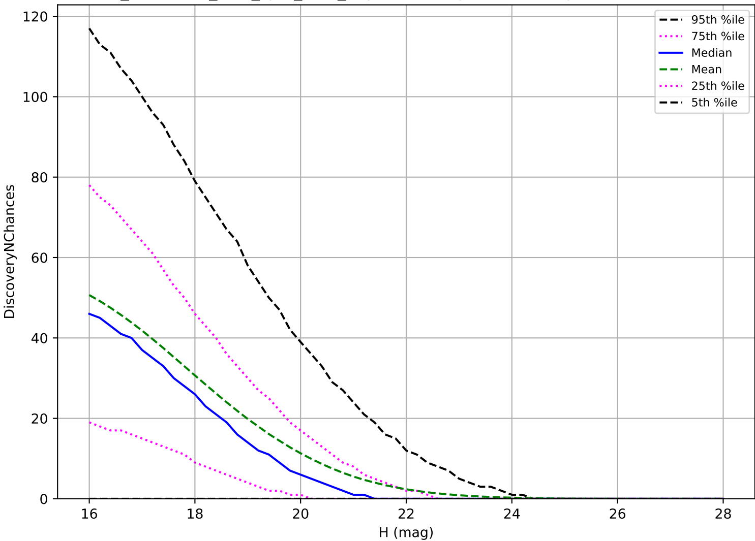
too_combined_s1.0_split_v3.4_10yrs: NEO 3 pairs in 15 nights detection loss
