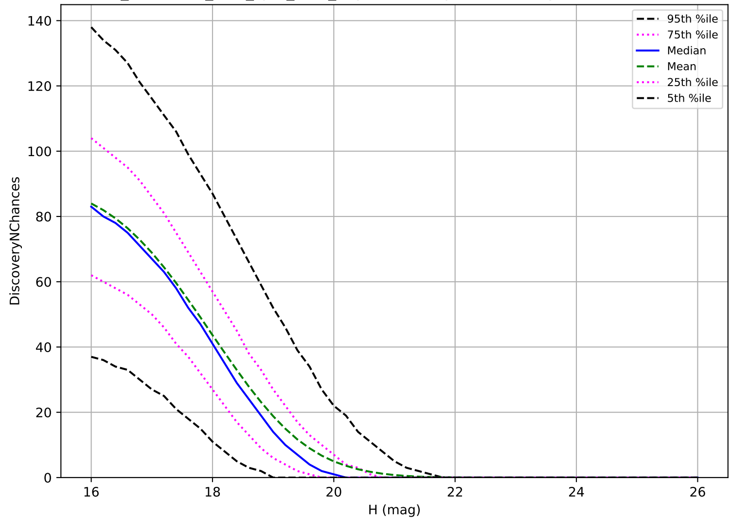
too_combined_s1.0_split_v3.4_10yrs: MBA 3 pairs in 15 nights detection loss
