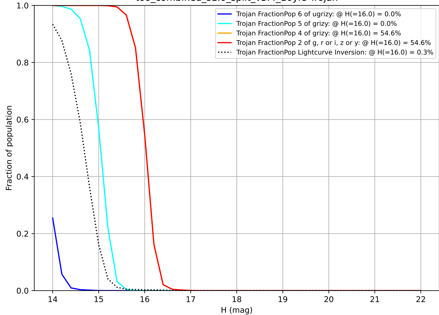
too_combined_s1.0_split_v3.4_10yrs Trojan
