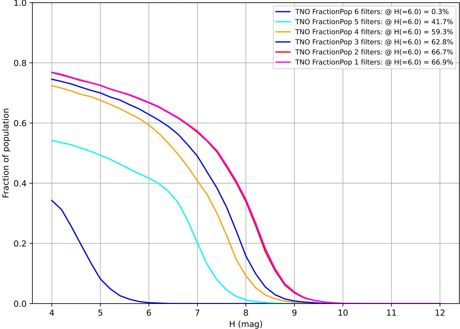
too_combined_s1.0_split_v3.4_10yrs: Fraction of population with colors in X filters TNO
