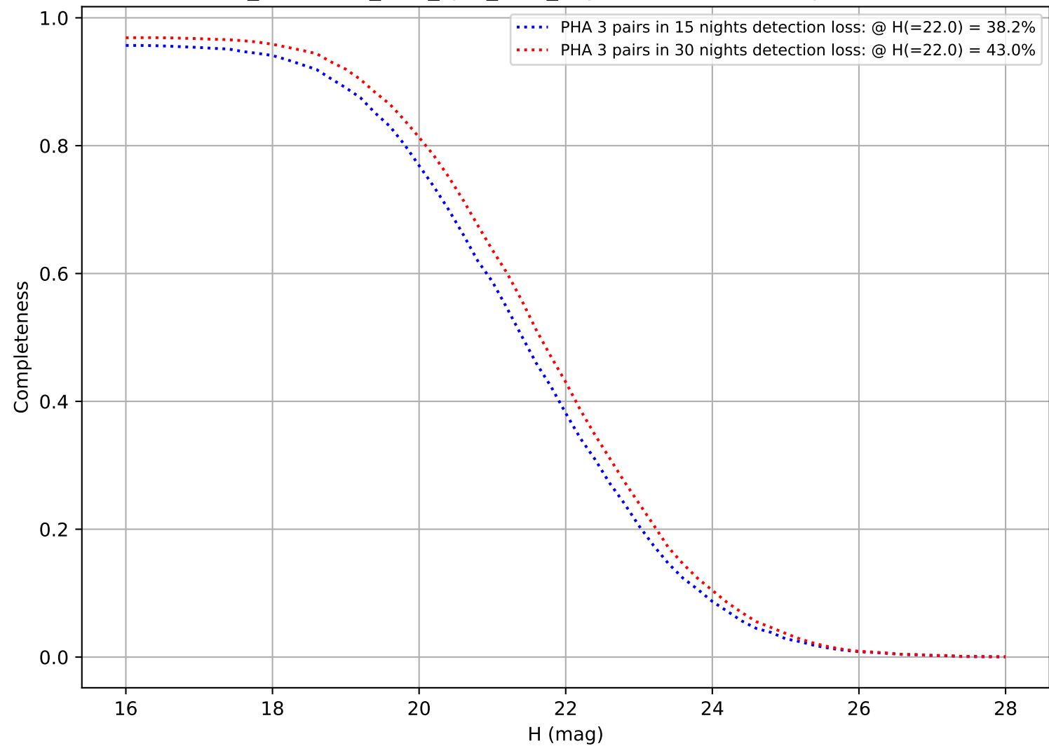
too_combined_s1.0_split_v3.4_10yrs: DifferentialCompleteness
