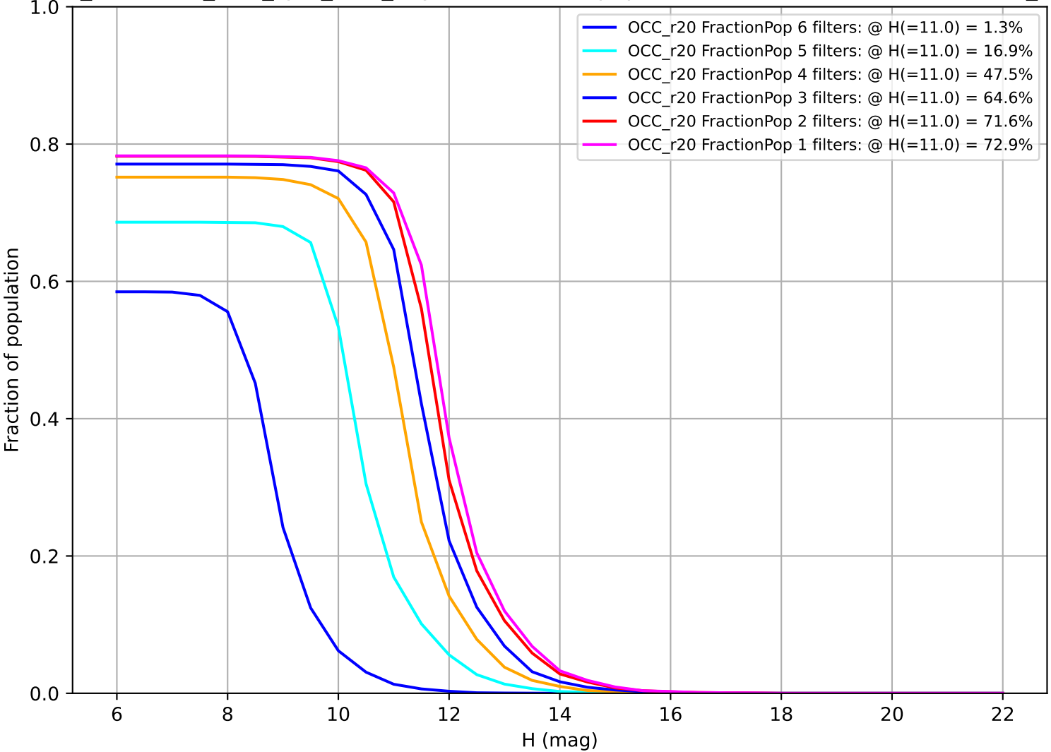
too_combined_s1.0_split_v3.4_10yrs: Fraction of population with colors in X filters OCC_r20
