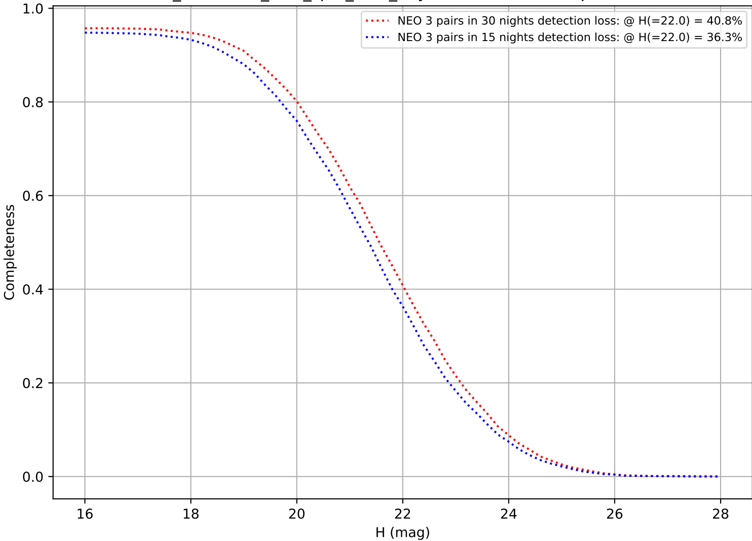
too_combined_s1.0_split_v3.4_10yrs: DifferentialCompleteness
