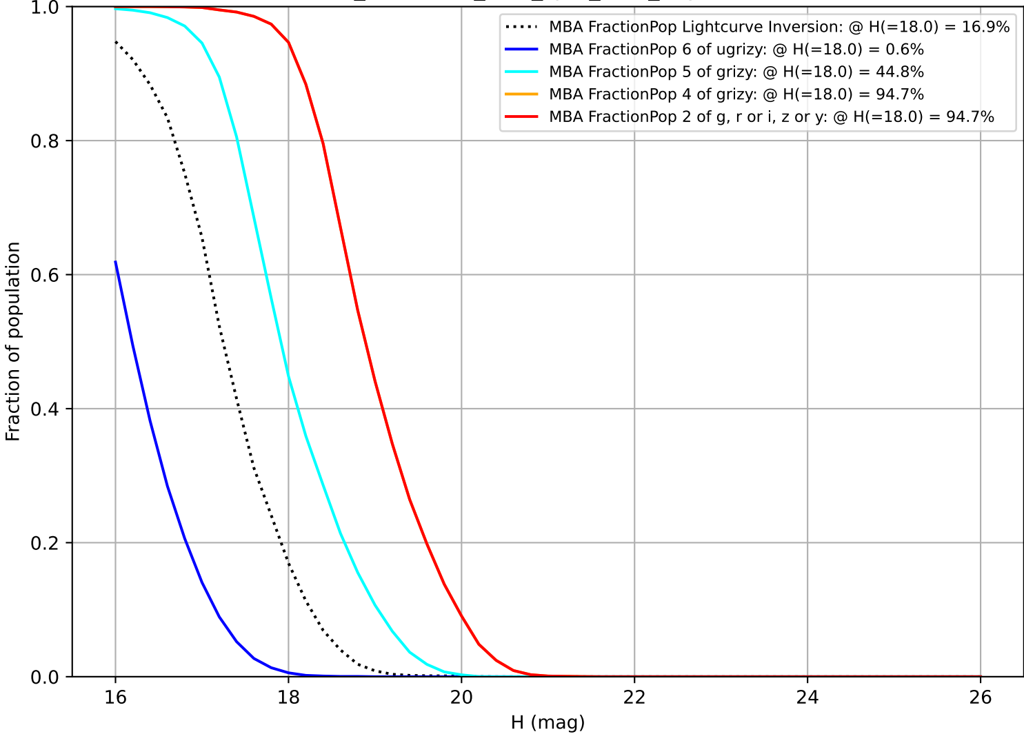
too_combined_s1.0_split_v3.4_10yrs MBA
