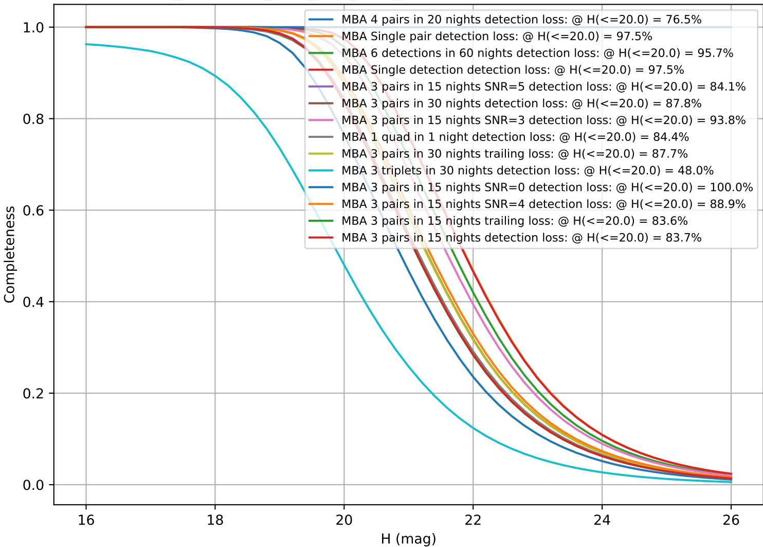
too_combined_s1.0_split_v3.4_10yrs: CumulativeCompleteness
