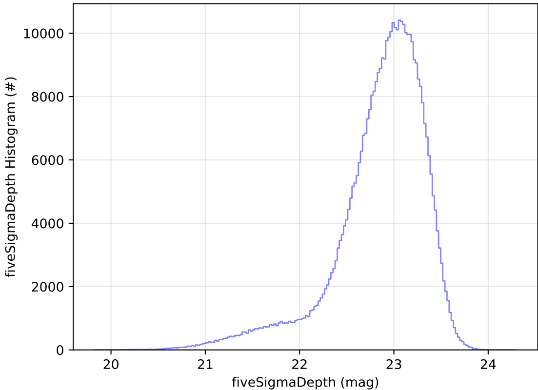
too_combined_s1.0_split_v3.4_10yrs z: fiveSigmaDepth Histogram
