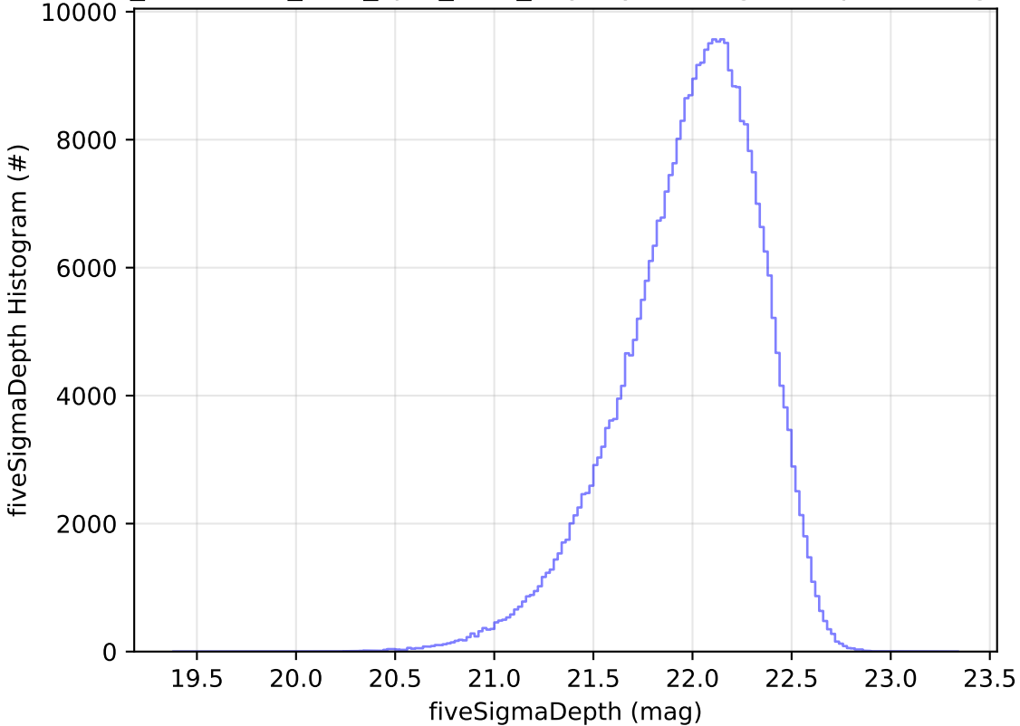
too_combined_s1.0_split_v3.4_10yrs y: fiveSigmaDepth Histogram
