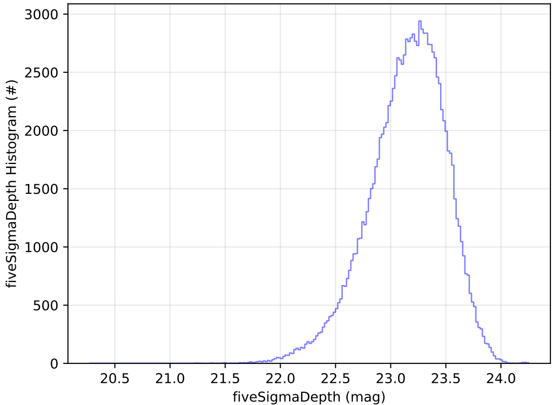
too_combined_s1.0_split_v3.4_10yrs u: fiveSigmaDepth Histogram
