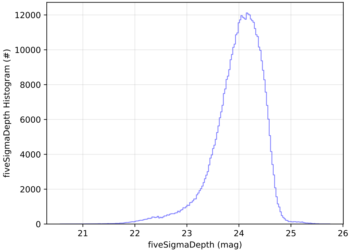
too_combined_s1.0_split_v3.4_10yrs r: fiveSigmaDepth Histogram
