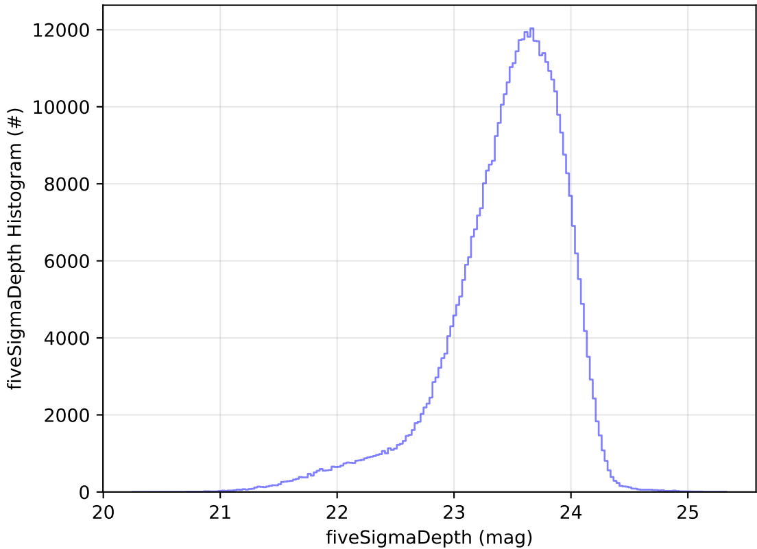
too_combined_s1.0_split_v3.4_10yrs i: fiveSigmaDepth Histogram
