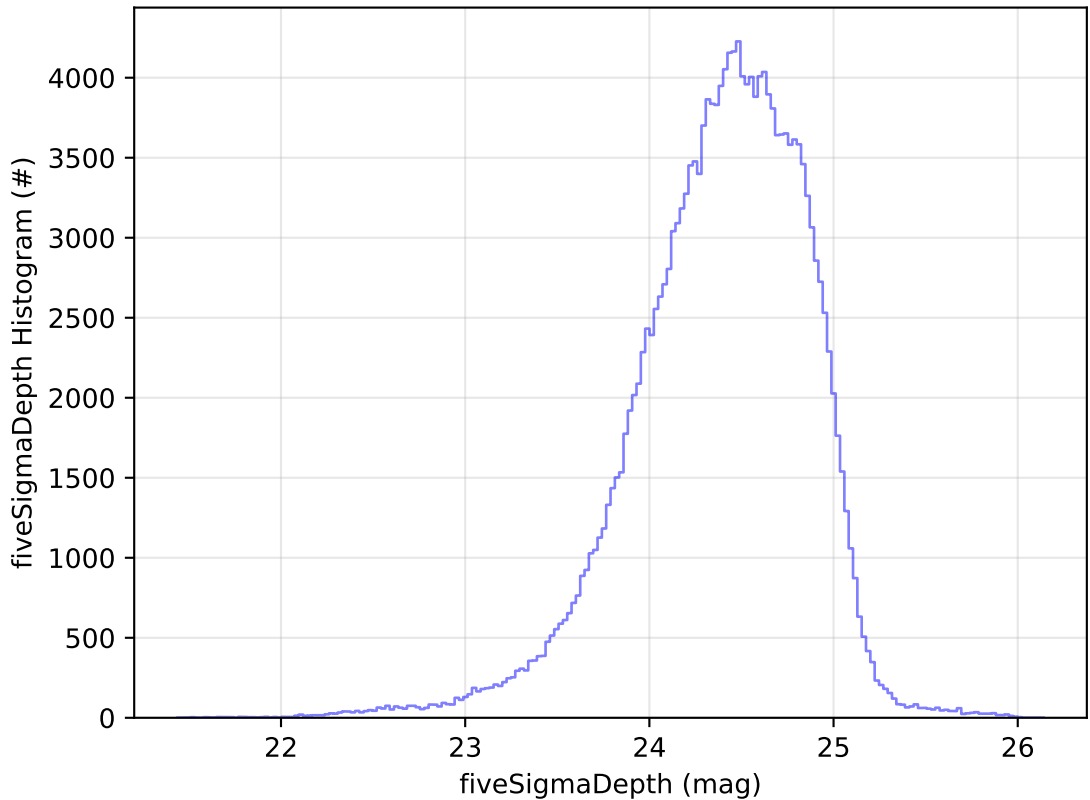
too_combined_s1.0_split_v3.4_10yrs g: fiveSigmaDepth Histogram
