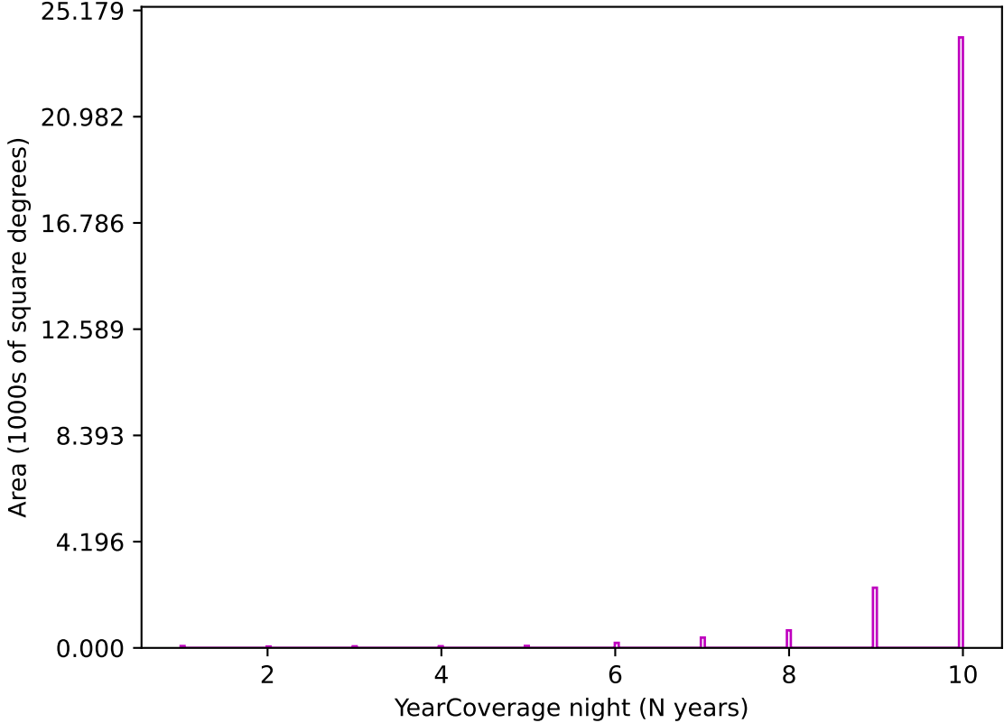
too_combined_s1.0_split_v3.4_10yrs z band: YearCoverage night
