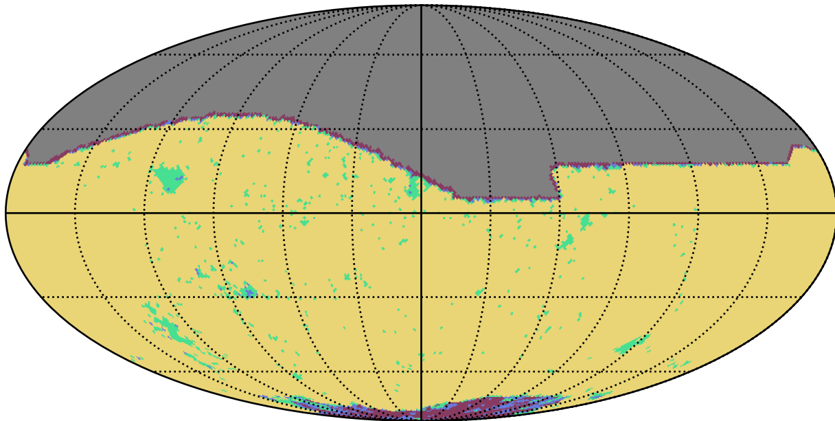
too_combined_s1.0_split_v3.4_10yrs i band: YearCoverage night
