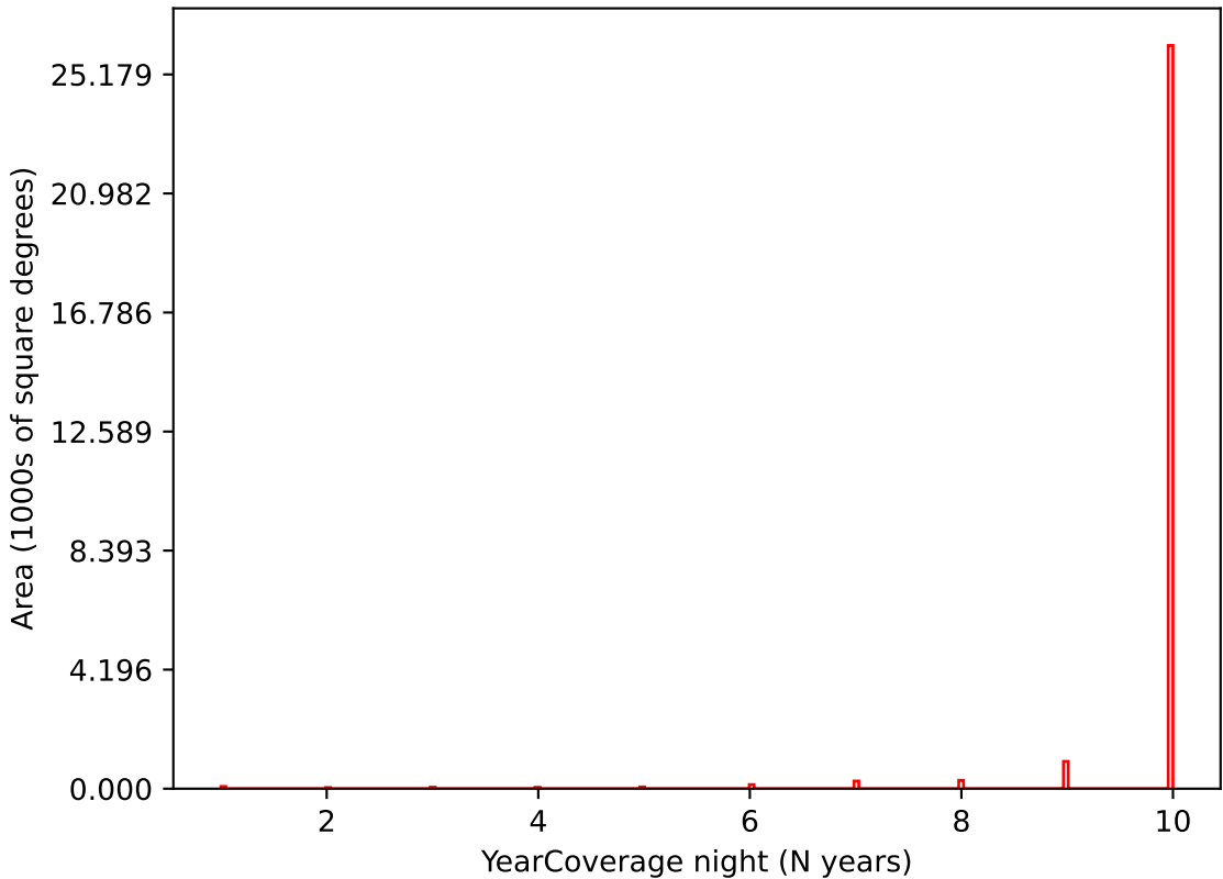
too_combined_s1.0_split_v3.4_10yrs i band: YearCoverage night
