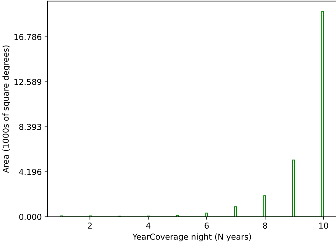
too_combined_s1.0_split_v3.4_10yrs g band: YearCoverage night
