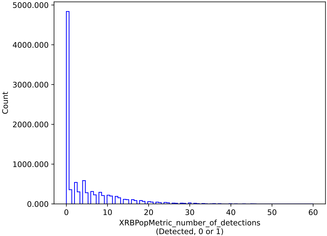
too_combined_s1.0_split_v3.4_10yrs : XRBPoMetric_number_of_detections
