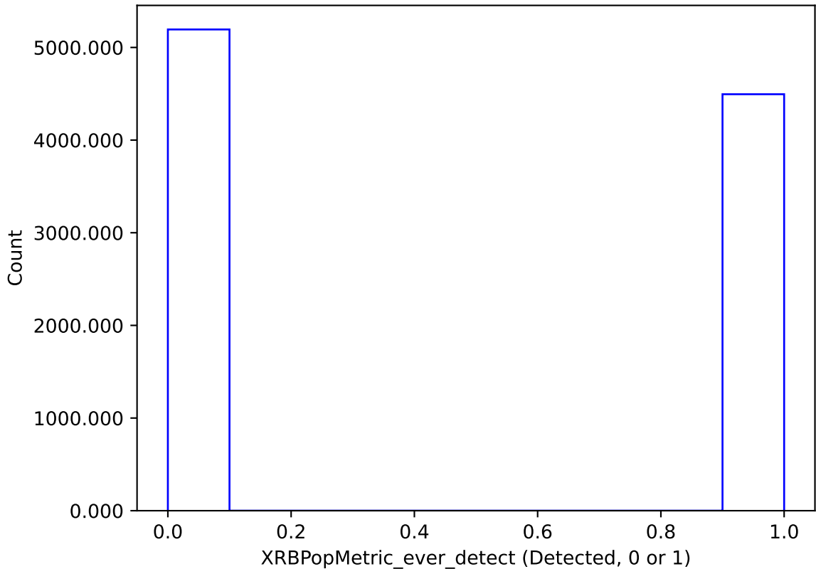
too_combined_s1.0_split_v3.4_10yrs : XRBPoMetric_ever_detect
