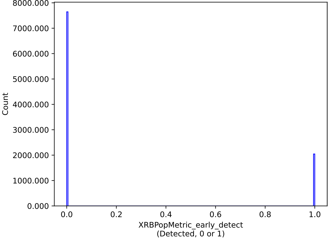
too_combined_s1.0_split_v3.4_10yrs : XRBPoMetric_early_detect
