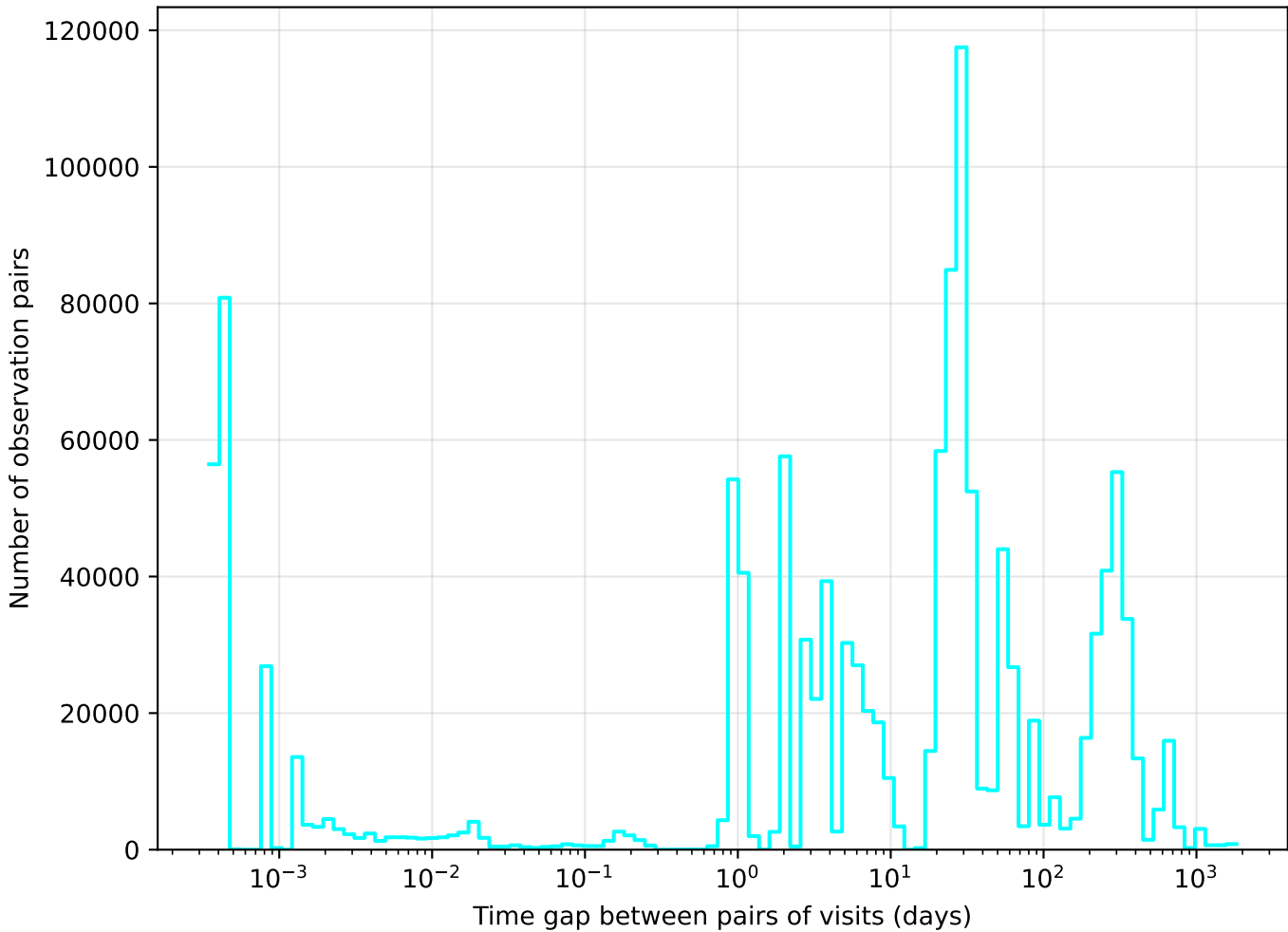
too_combined_s1.0_split_v3.4_10yrs u band: Tgaps observationStartMJD
