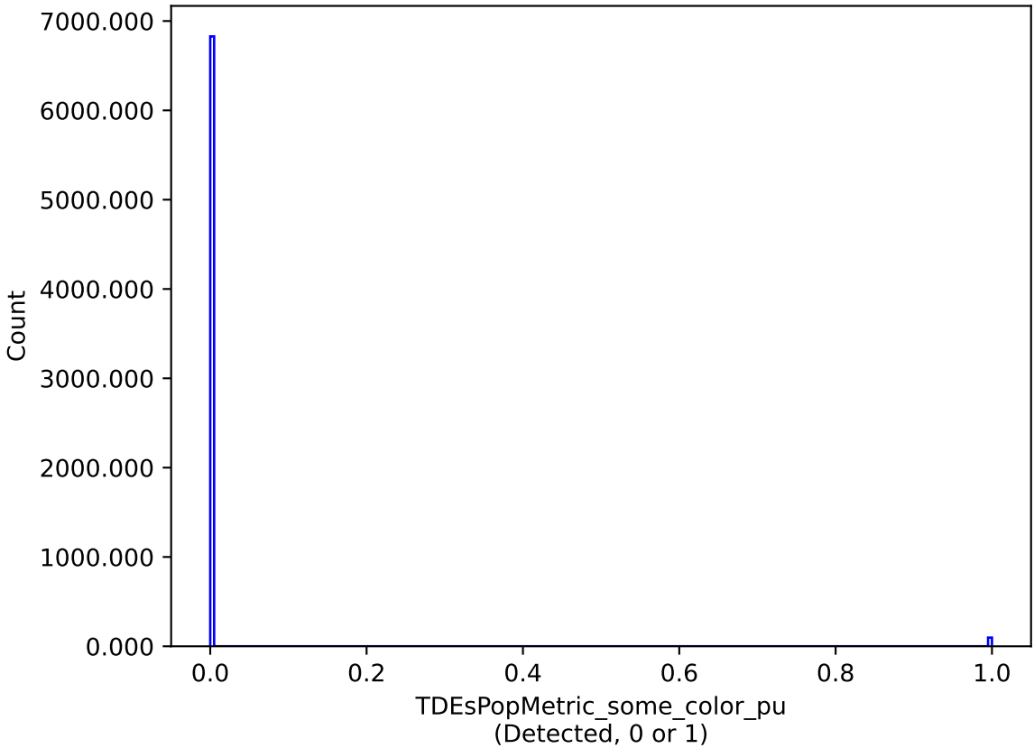
too_combined_s1.0_split_v3.4_10yrs : TDEsPopMetric_some_color_pu
