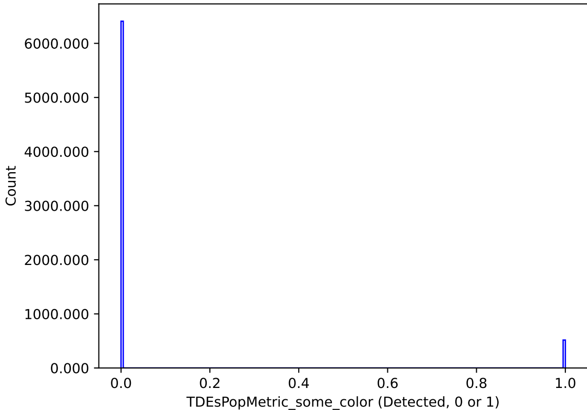
too_combined_s1.0_split_v3.4_10yrs : TDEsPopMetric_some_color
