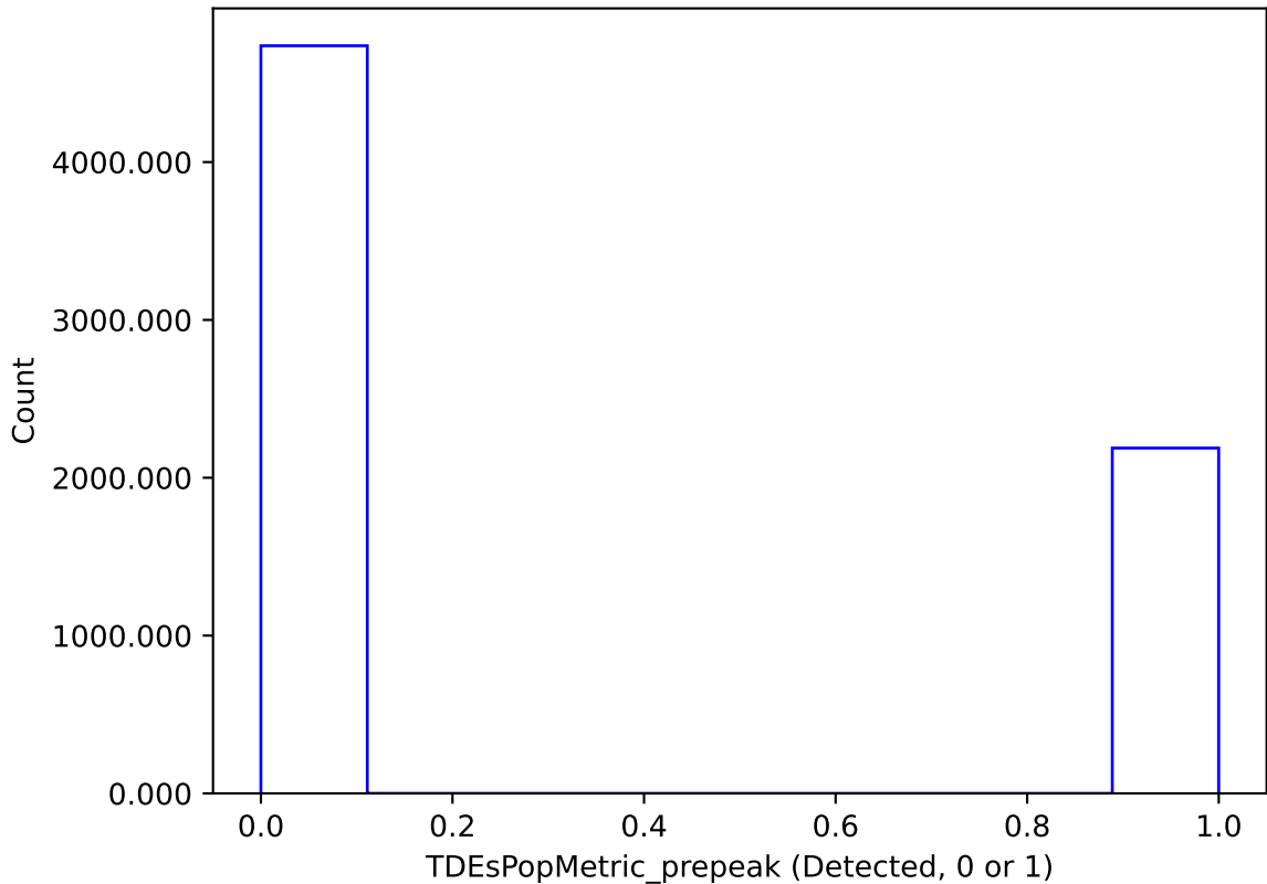
too_combined_s1.0_split_v3.4_10yrs : TDEsPopMetric_prepeak
