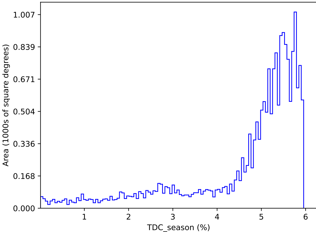
too_combined_s1.0_split_v3.4_10yrs : TDC_season
