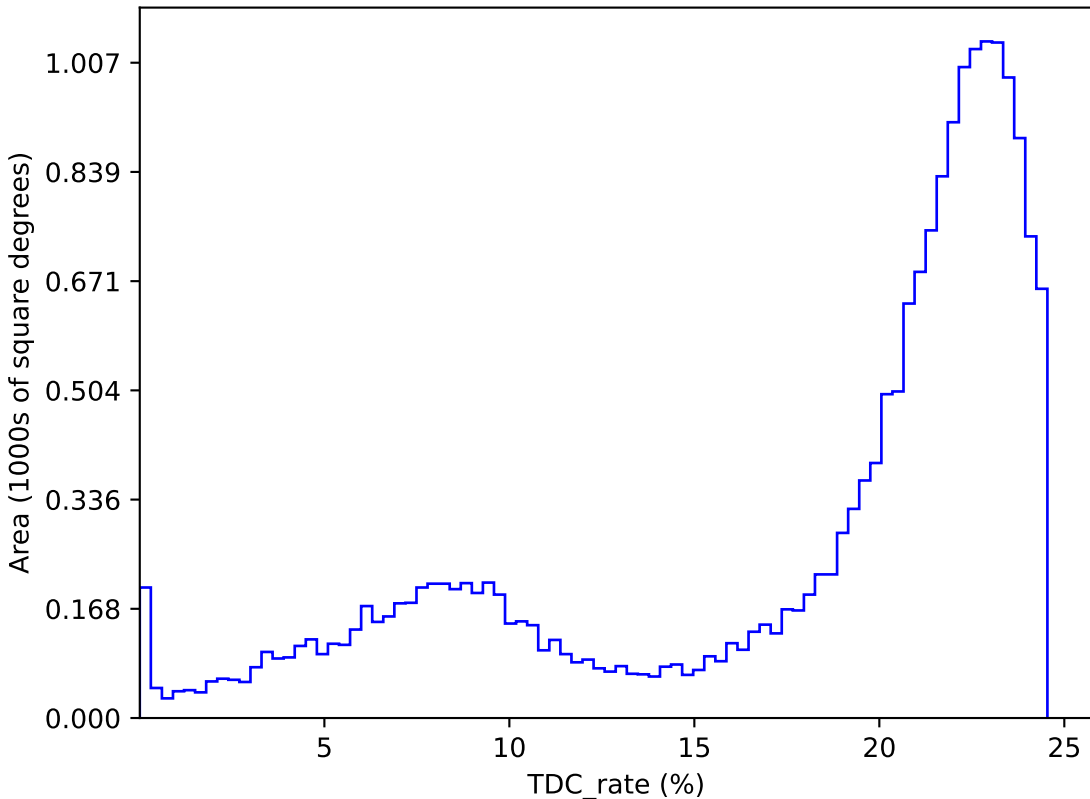
too_combined_s1.0_split_v3.4_10yrs : TDC_rate
