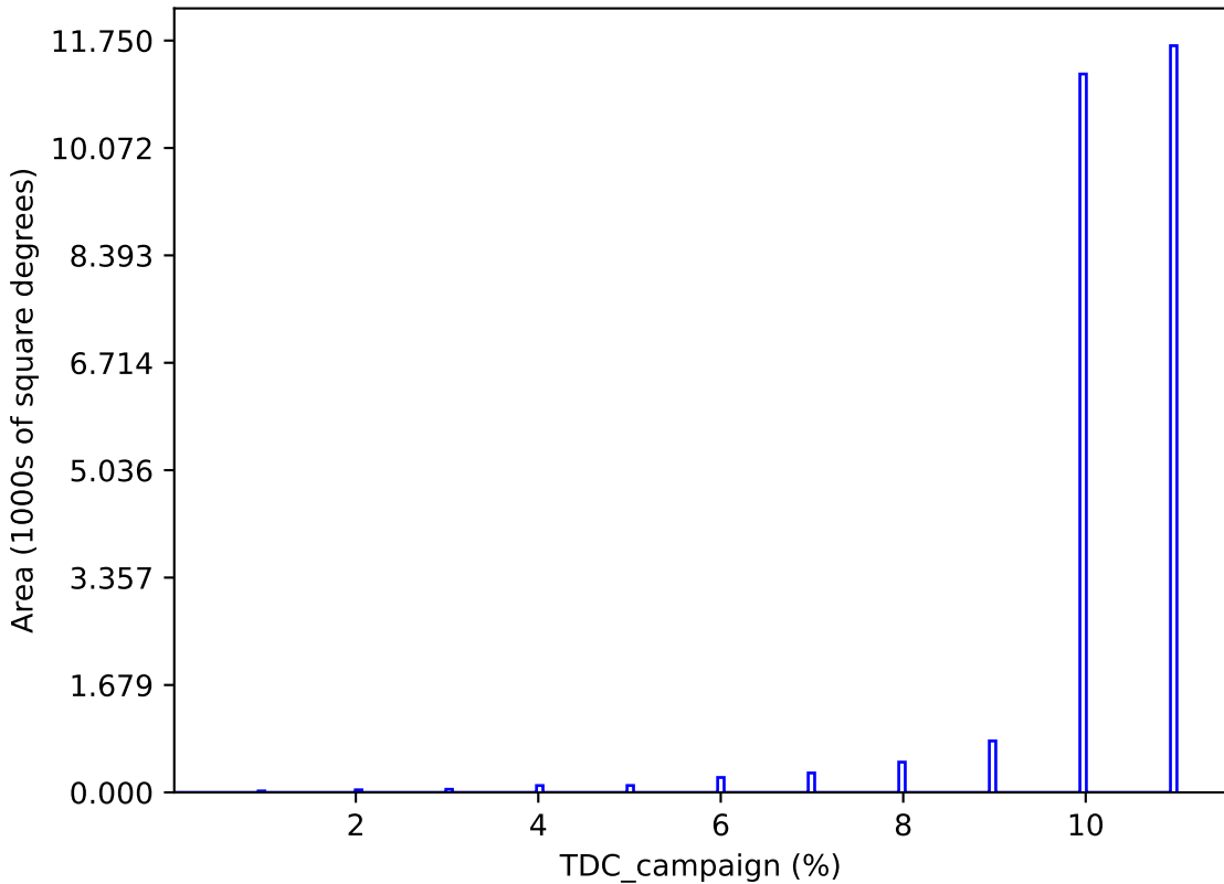
too_combined_s1.0_split_v3.4_10yrs : TDC_campaign
