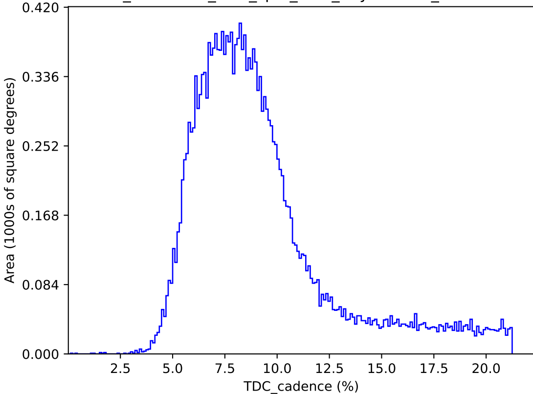
too_combined_s1.0_split_v3.4_10yrs : TDC_cadence
