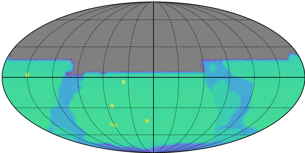
too_combined_s1.0_split_v3.4_10yrs y: SurfaceBrightLimit
