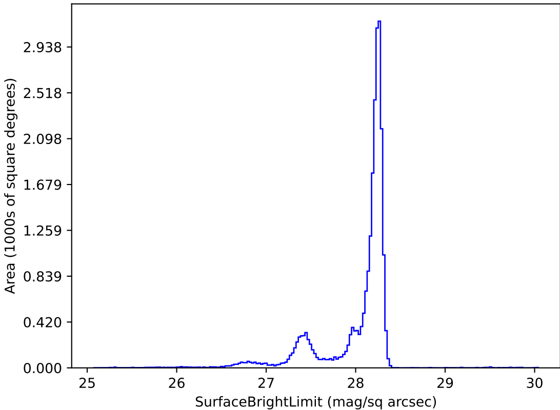
too_combined_s1.0_split_v3.4_10yrs y: SurfaceBrightLimit
