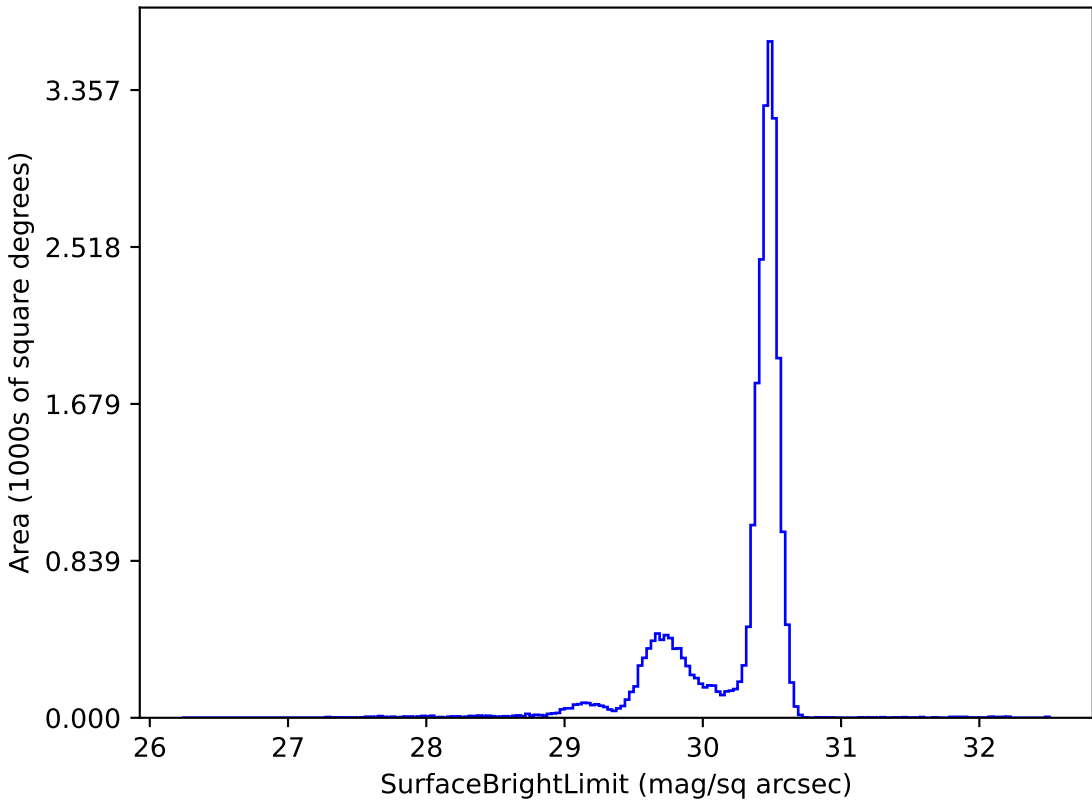
too_combined_s1.0_split_v3.4_10yrs r: SurfaceBrightLimit
