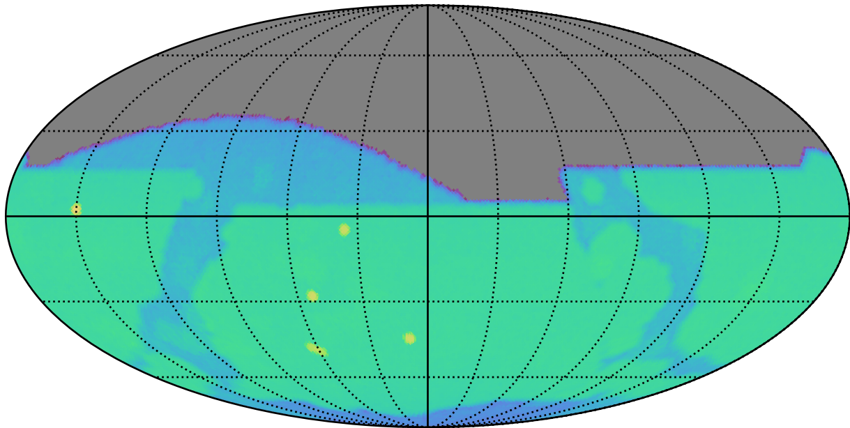
too_combined_s1.0_split_v3.4_10yrs i: SurfaceBrightLimit
