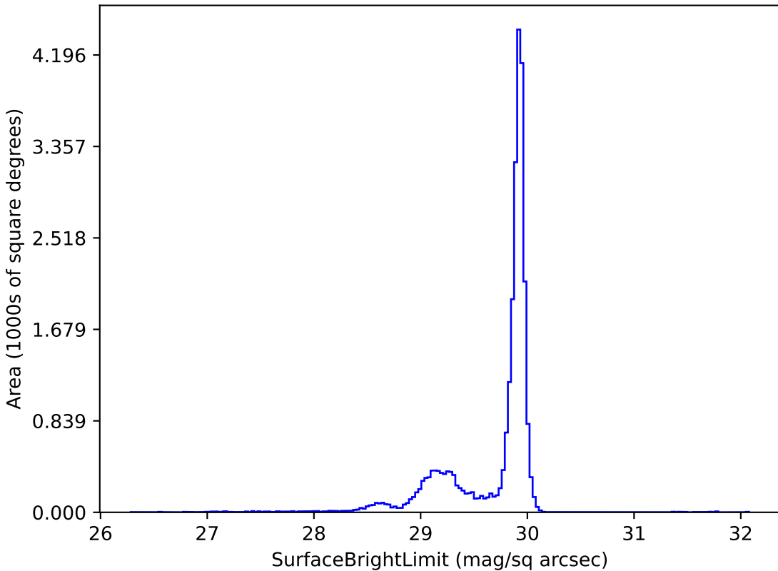
too_combined_s1.0_split_v3.4_10yrs i: SurfaceBrightLimit
