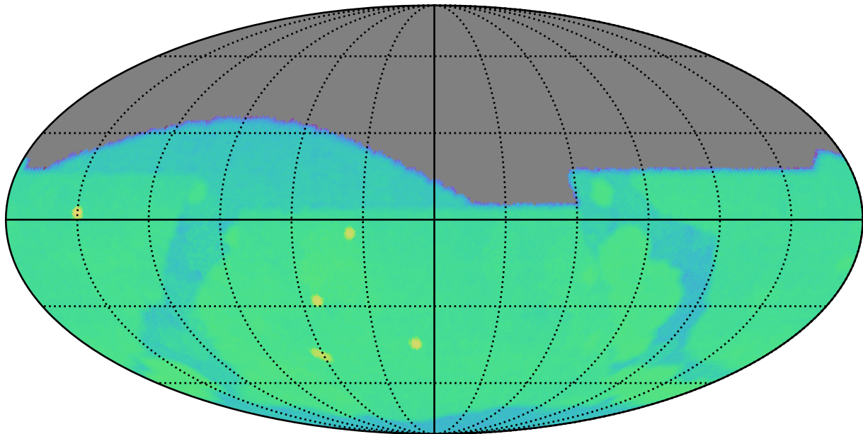
too_combined_s1.0_split_v3.4_10yrs g: SurfaceBrightLimit
