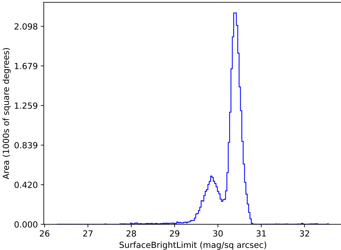
too_combined_s1.0_split_v3.4_10yrs g: SurfaceBrightLimit
