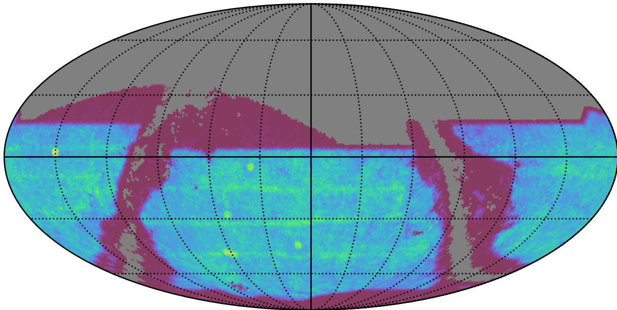
too_combined_s1.0_split_v3.4_10yrs : SNSLMetric
