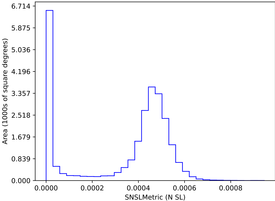
too_combined_s1.0_split_v3.4_10yrs : SNSLMetric
