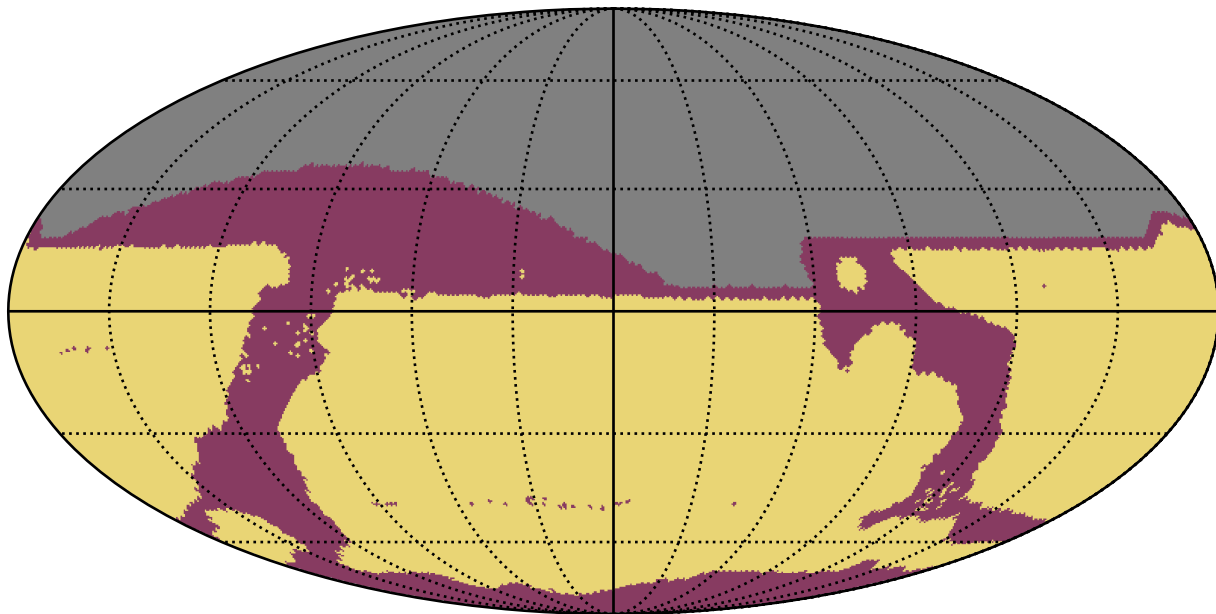
too_combined_s1.0_split_v3.4_10yrs : RapidRevisits
