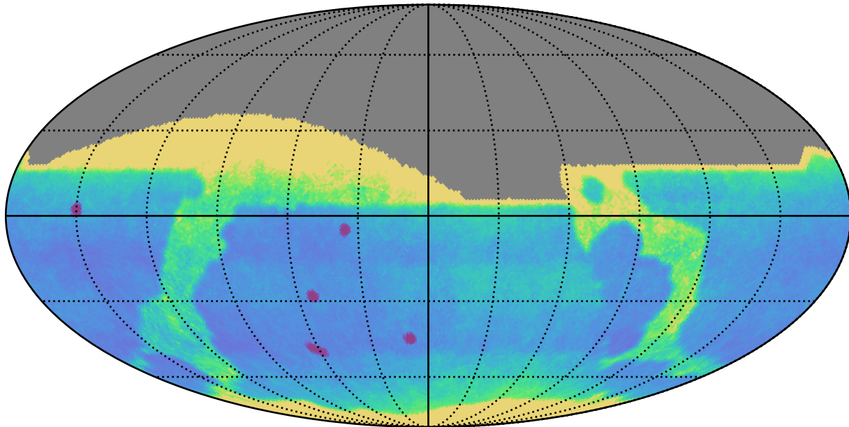
too_combined_s1.0_split_v3.4_10yrs : Proper Motion Uncert @ 24.0
