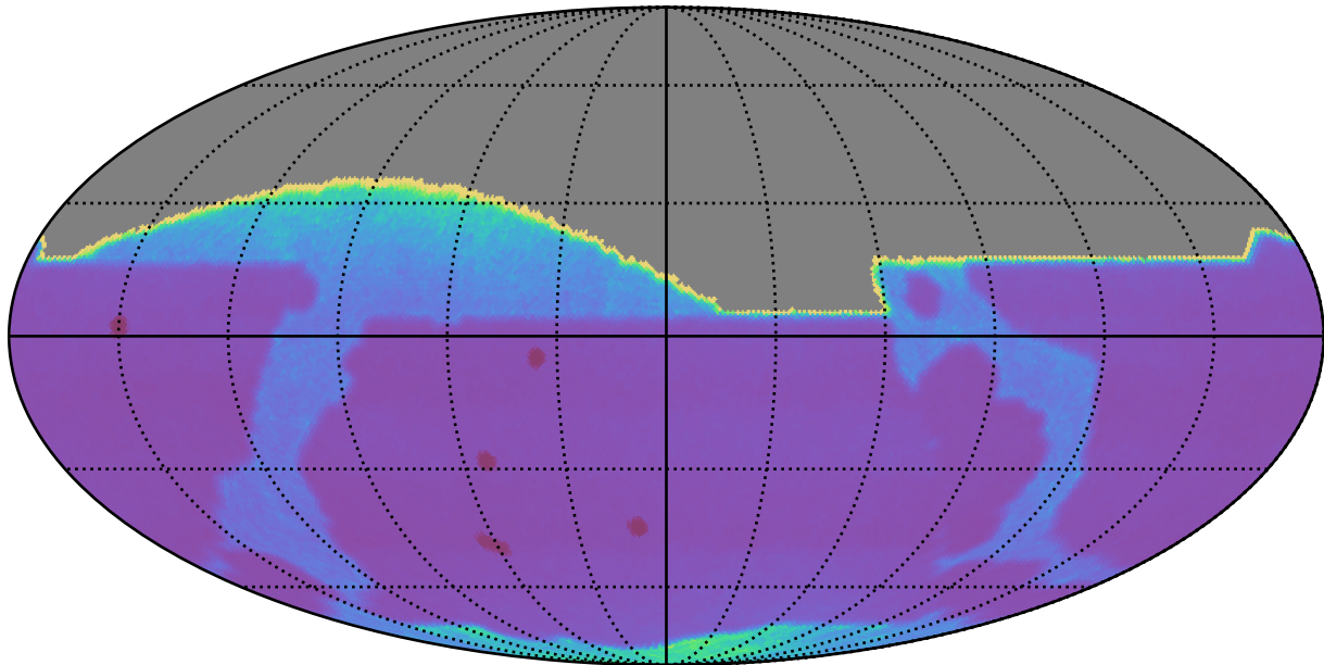
too_combined_s1.0_split_v3.4_10yrs : Proper Motion Uncert @ 20.5
