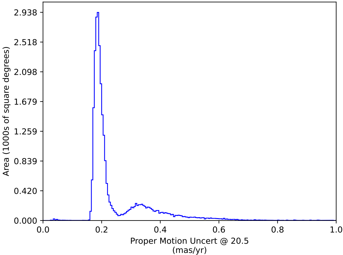
too_combined_s1.0_split_v3.4_10yrs : Proper Motion Uncert @ 20.5
